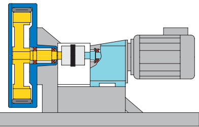
Long-coupled
