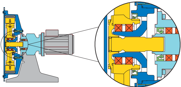
Bredel direct-coupled
